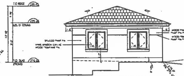
5 NORTH ELEVATION SCALE: 1/4" = 1'-0"
