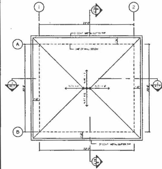
2 ROOF PLAN SCALE: 1/4" = 1'-0"
