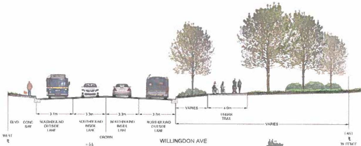
Fig. 1: Typical Section
