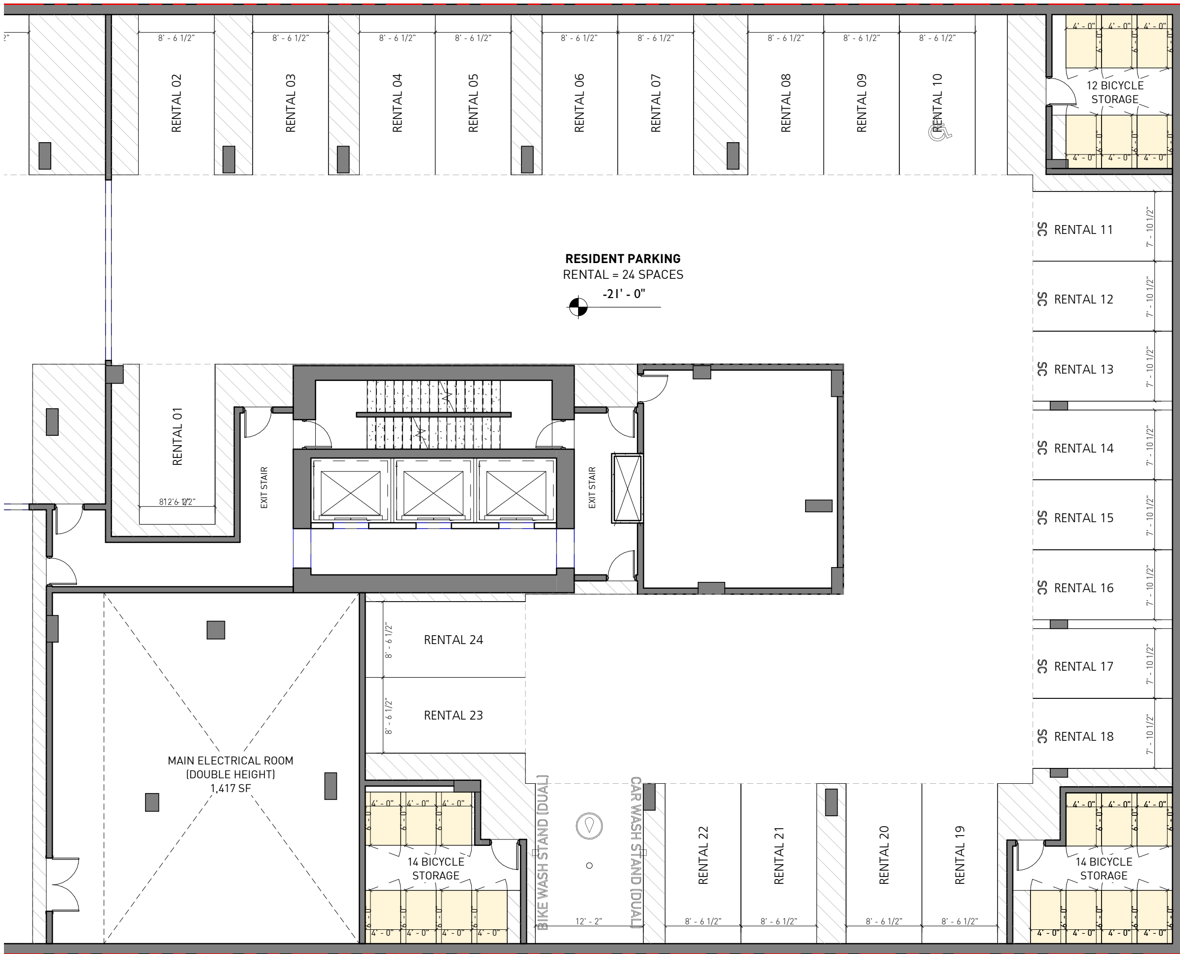
PARKING P2 - BICYCLE FACILITY STANDARDS 3/32" = 1'-0"
