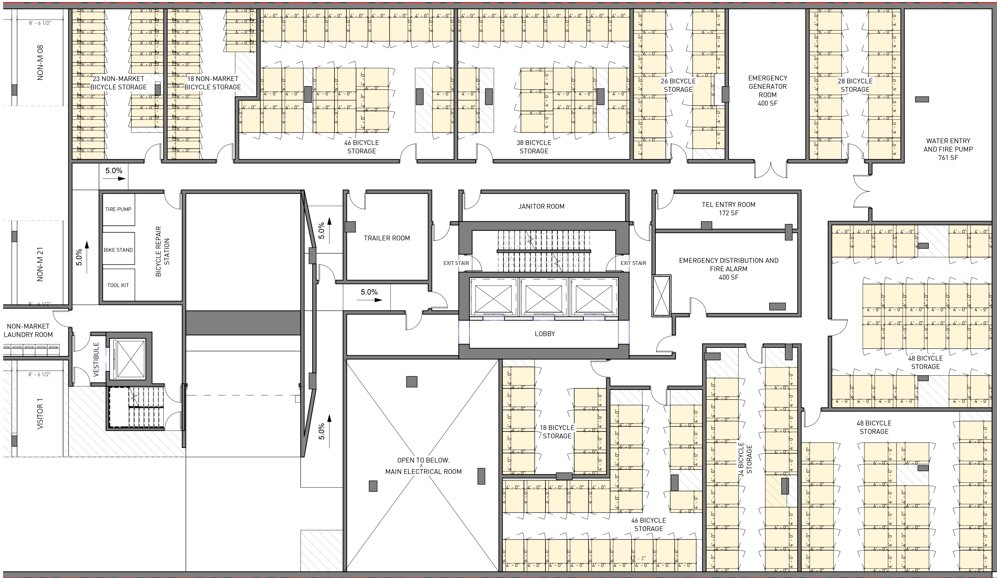
PARKING P1 - BICYCLE FACILITY STANDARDS 3/32" = 1'-0"
