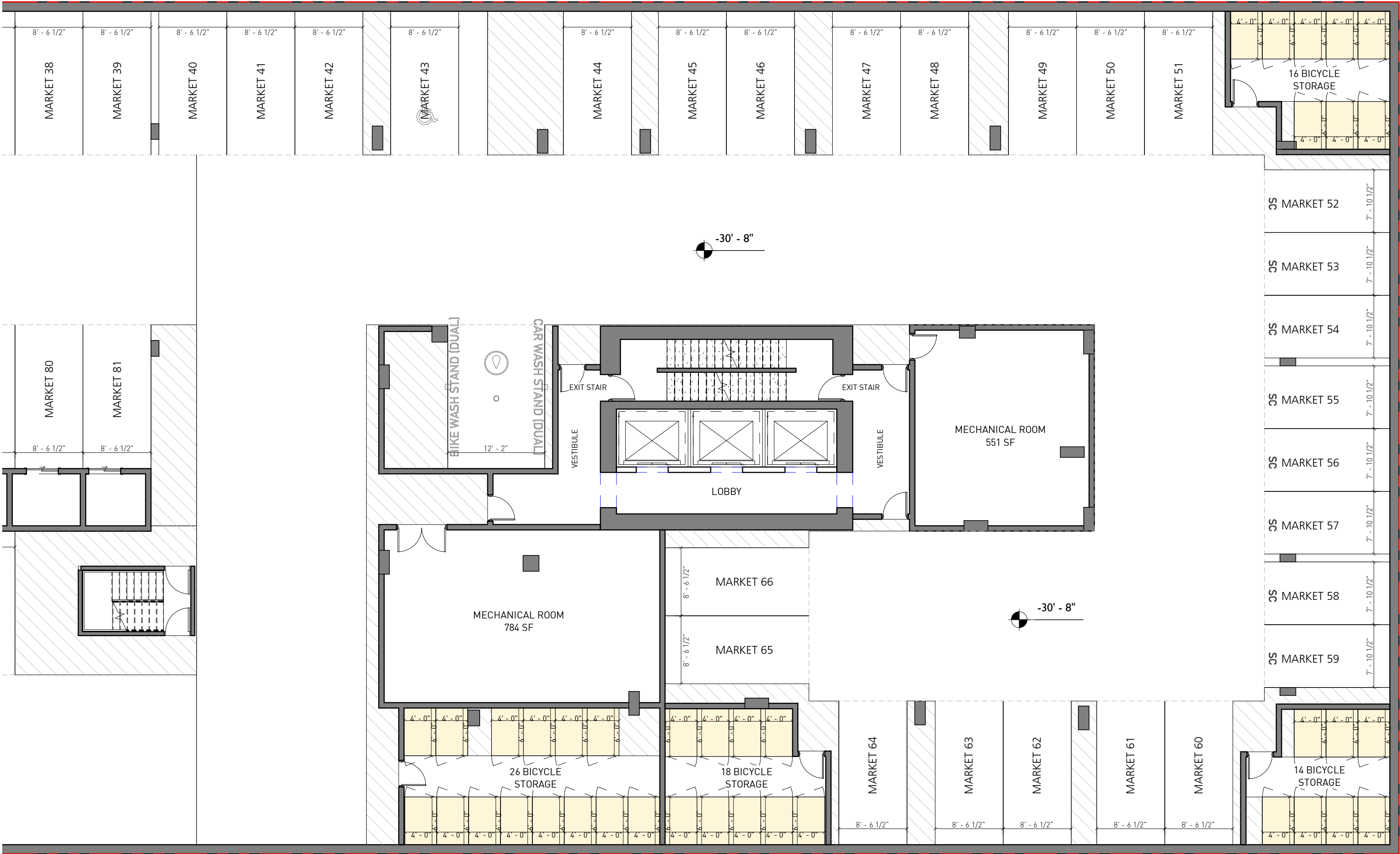
PARKING P3 - BICYCLE FACILITY STANDARDS 3/32" = 1'-0"
