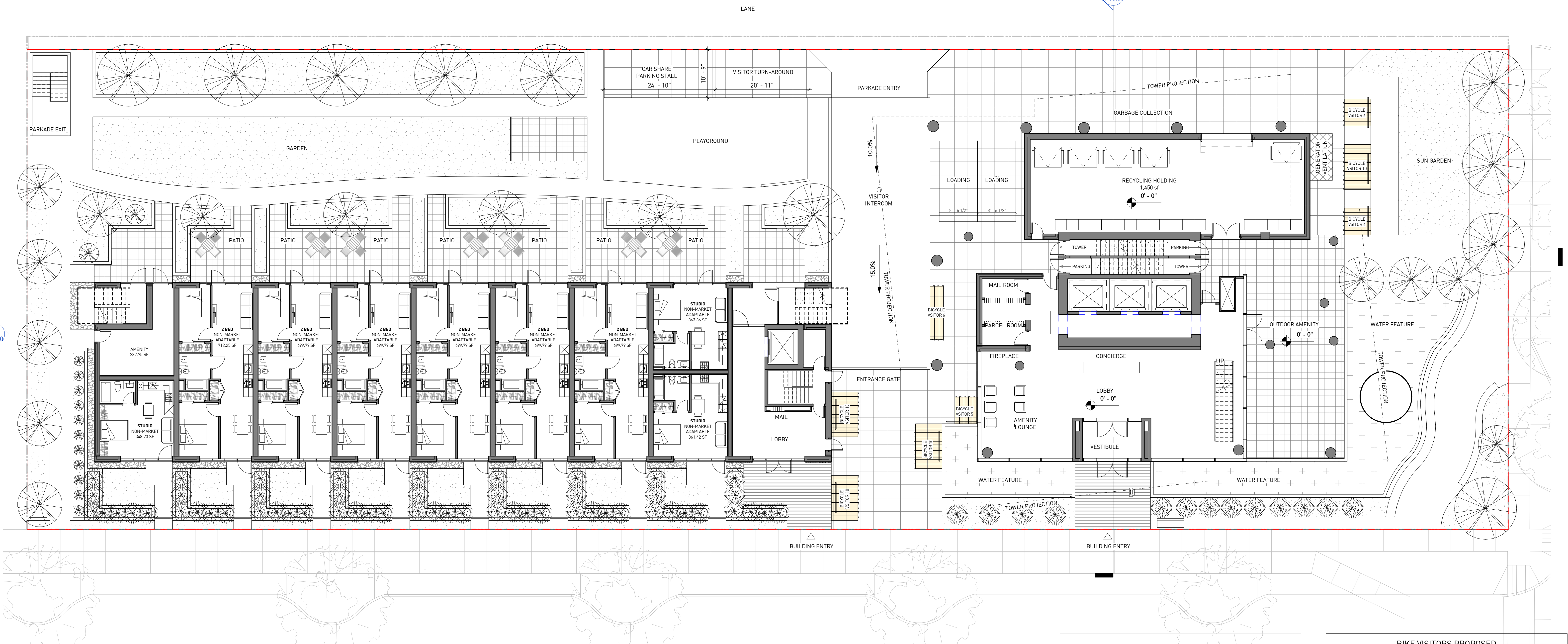
LEVEL 1 - OFF-STREET BICYCLE PARKING 3/32" = 1'-0"
