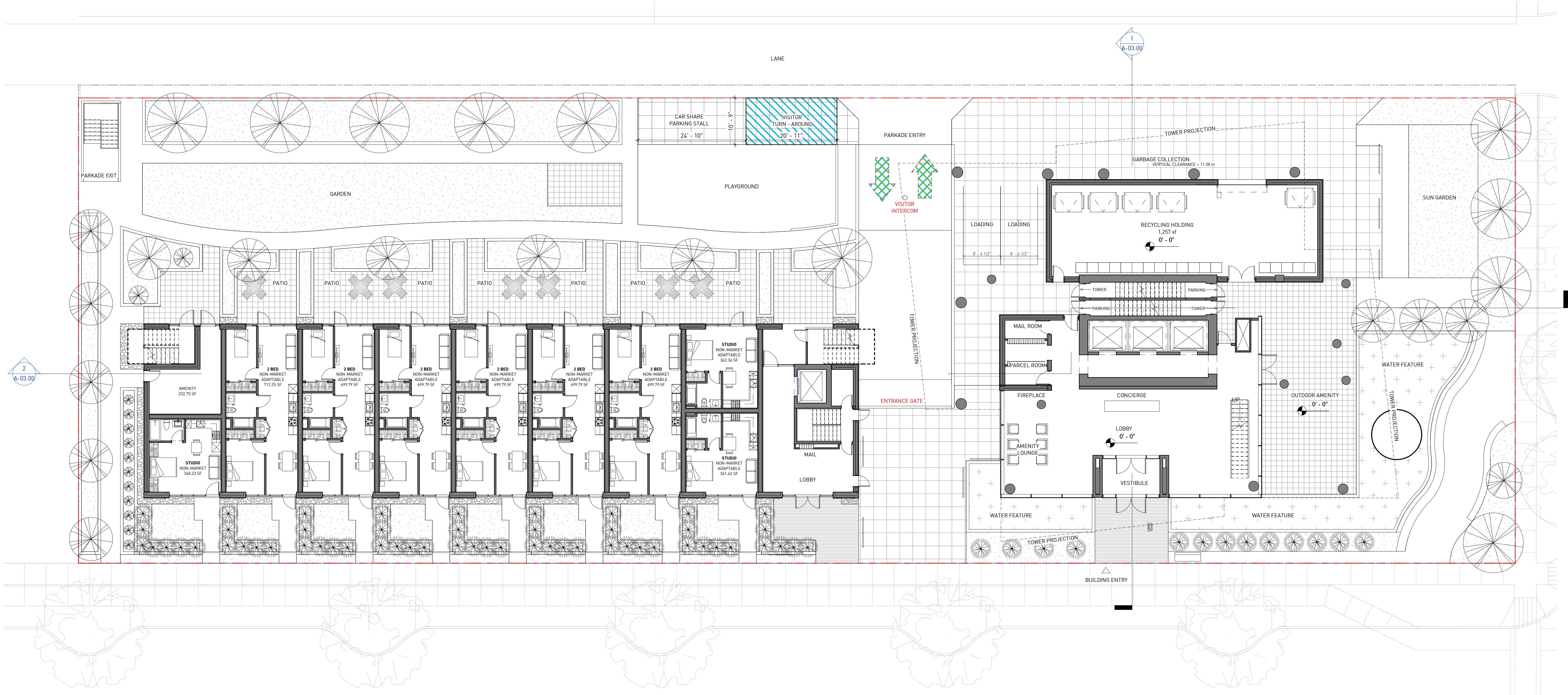
LEVEL 1 - VISITOR GATE ACCESS AND TURN-AROUND PLAN 3/32" = 1'-0"
