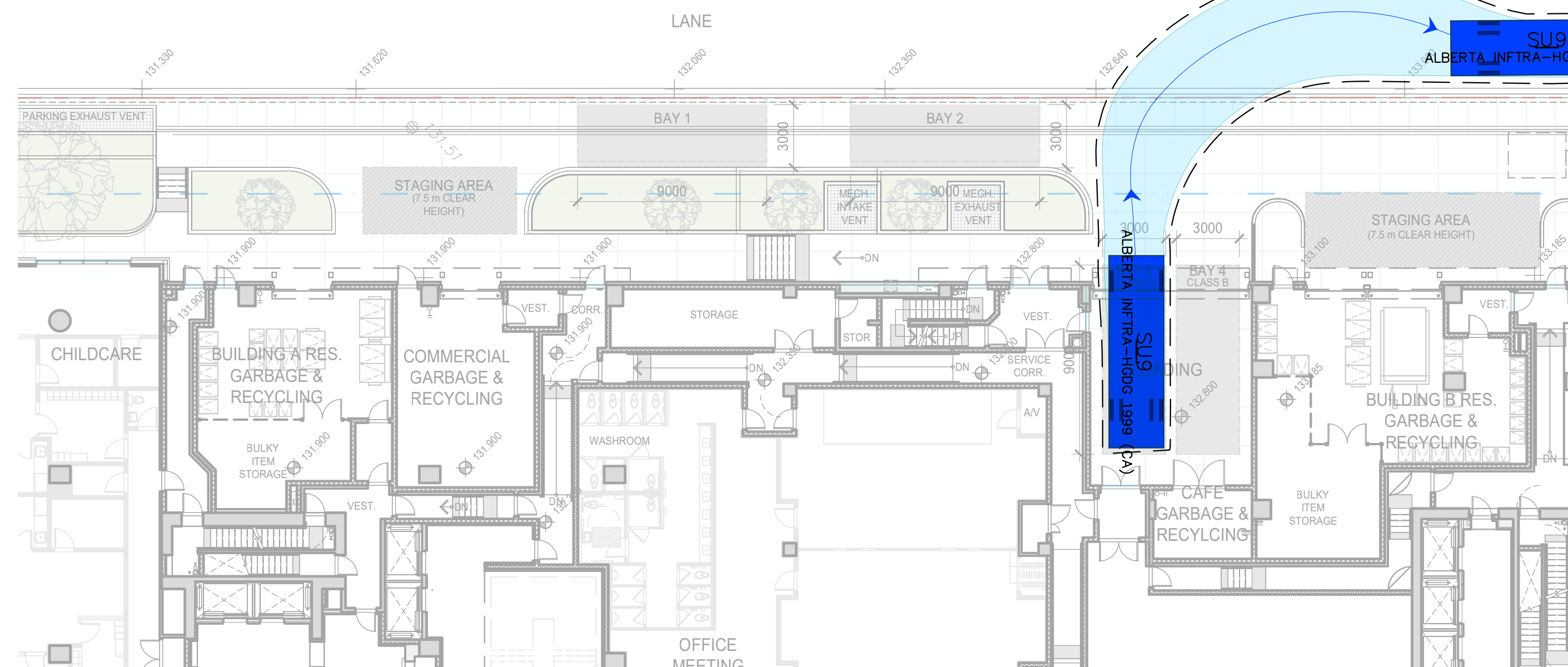
2 LOADING BAY 3 - VEHICLE EXITING MANEUVER 1:200
