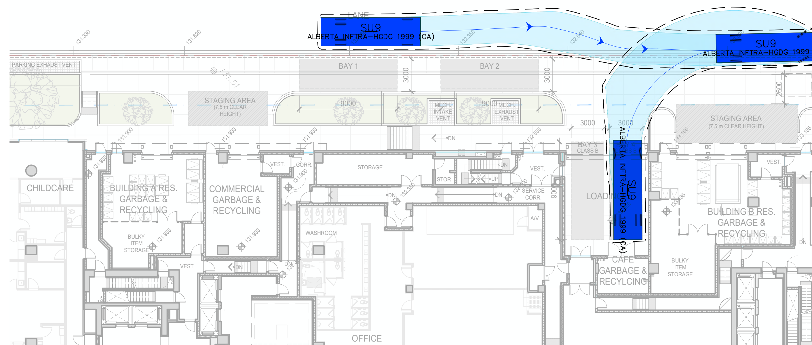
3 LOADING BAY 4 - VEHICLE PARKING MANEUVER 1:200
