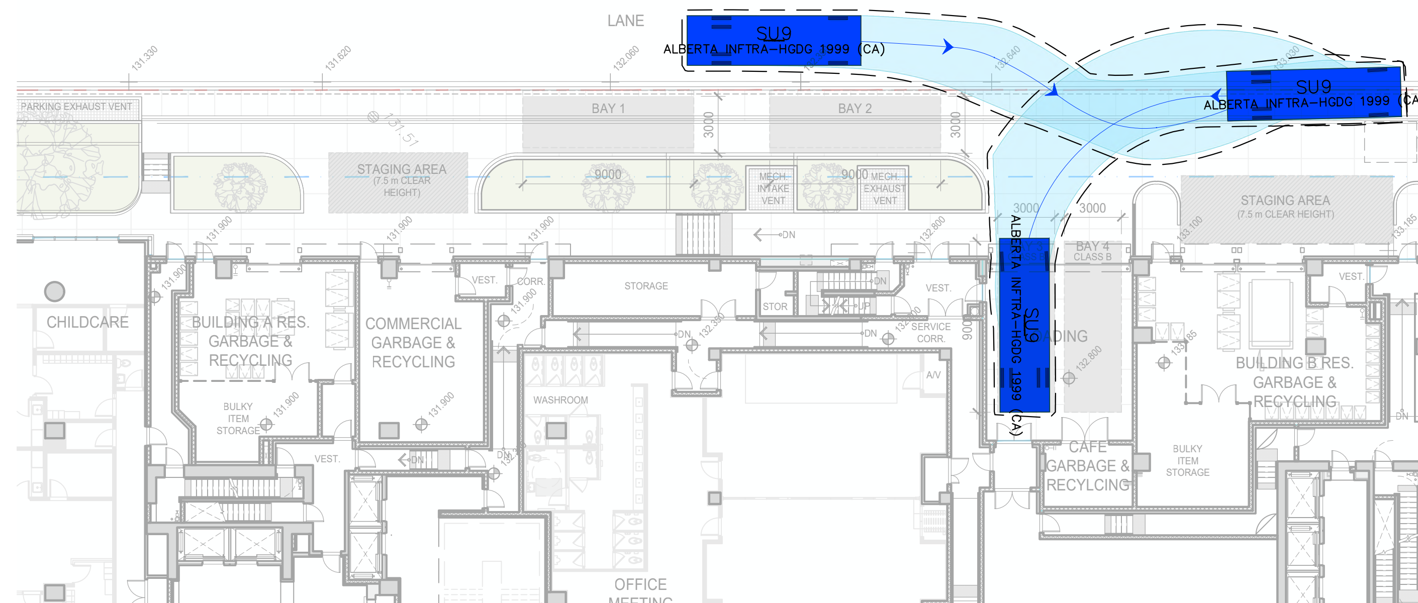
1 LOADING BAY 3 - VEHICLE PARKING MANEUVER 1:200
