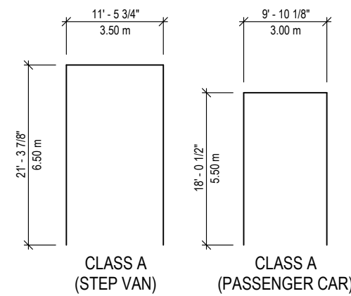
Bunt Recommended Loading Space Dimensions
