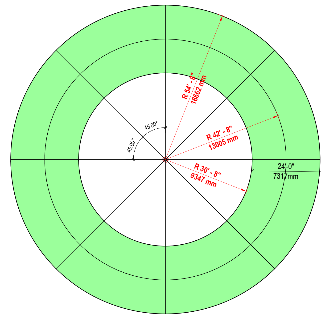
CITY OF BURNABY FIRE TRUCK TURNING RADIUS
