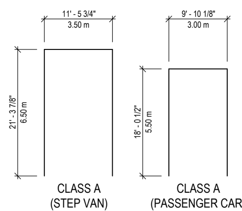
Bunt Recommended Loading Space Dimensions
