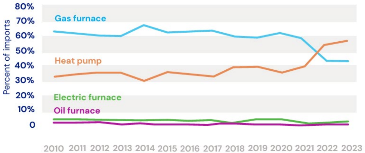
Figure 2: BC Shipment Data: Residential forced air heating equipment. Government of British Columbia, CleanBC Independent Review: Final Report (November 2025).
